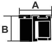
LA205SF SUPPORTO SQUARE SOFFITTO SQUARE CEILING BRACKET
