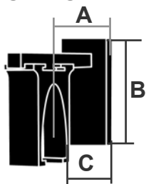
LA203 SUPPORTO DROP / DROP BRACKET
